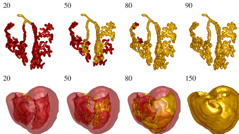
Fig. 5. Normal activation sequence. Time is counted in ms from the moment the upper part of the His bundle is stimulated. In the top row, only the propagation of the wave through the Purkinje system is displayed. In the bottom row, propagation through the Purkinje system and ventricles is displayed. Snapshots are taken at the indicated times. (Top row) Normal activation sequence in the Purkinje system. (Bottom row) Normal activation sequence in the ventricles and Purkinje system.
